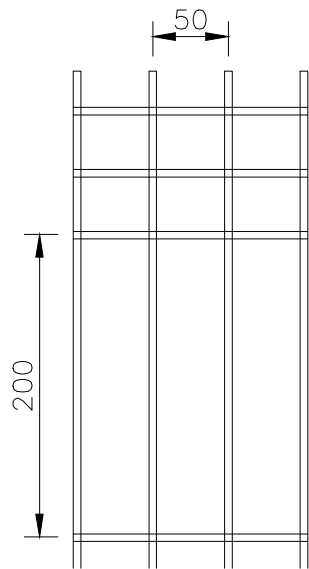
MESH DETAILS (SCALE 1:5)
