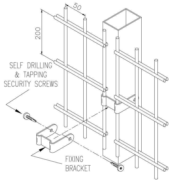
FIXING DETAILS
