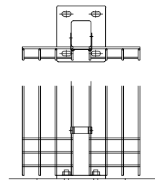
BASEPLATE SLOTTED FOR M12 CHEMICAL FIXINGS
