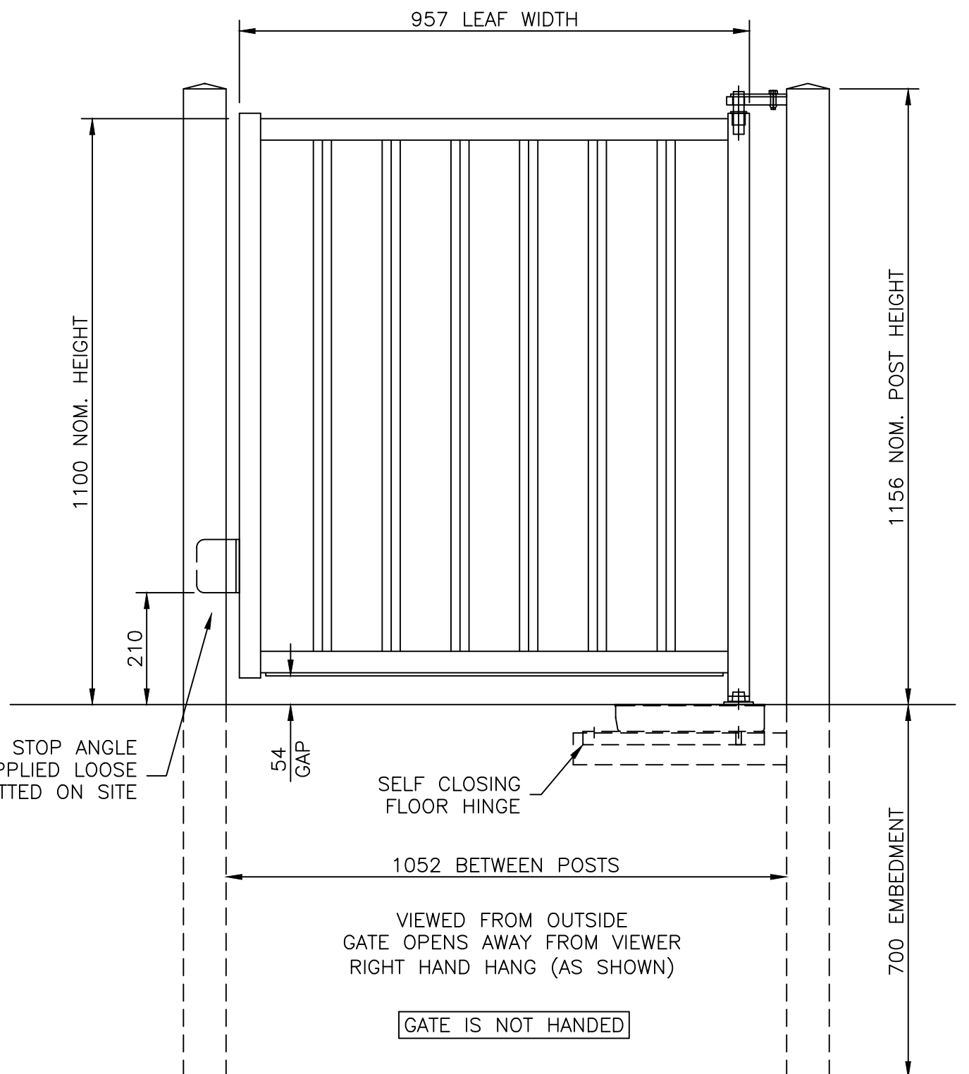
MULTI-COLOURD PLAYTIME METAL SELF CLOSING GATE
